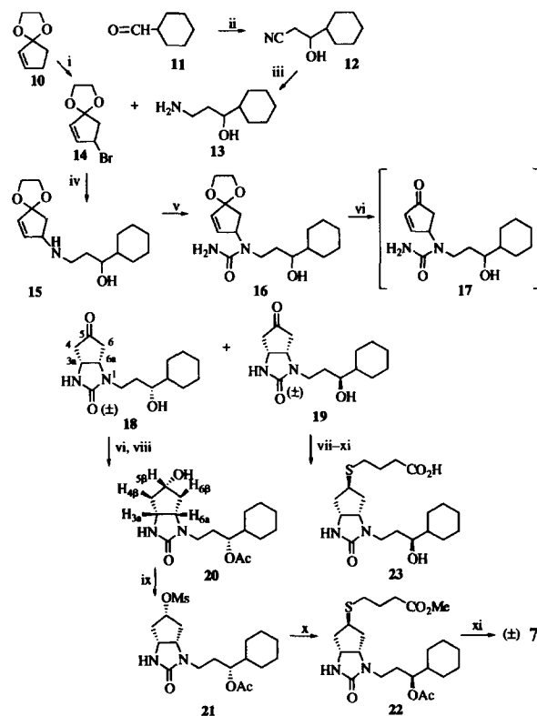
Scheme 1. Reagents: (i) NBS, AIBN, \text{CCl}_4 [ref. 15]; (ii) n\text{-BuLi} , \text{CH}_3\text{CN} , -78^\circ\text{C} (52%); (iii) \text{LiAlH}_4 , \text{Et}_2\text{O} , 25^\circ\text{C} (58%); (iv) Toluene, 25^\circ\text{C} for 24 h; 40^\circ\text{C} for 3 h; \text{NEt}_3 (32%); (v) \text{KCNO} , 1 N \text{HCl} , \text{EtOH-H}_2\text{O} (85%); (vi) 2 N \text{HCl} , \text{THF} , 25^\circ\text{C} , 2 h (45% of 18 ; 40% of 19 ); (vii) \text{Ac}_2\text{O} , \text{C}_6\text{H}_5\text{N} , rt, 18 h (84%); (viii) \text{NaBH}_4 , \text{EtOH} (54%); (ix) \text{MeSO}_2\text{Cl} , \text{C}_6\text{H}_5\text{N} , 0-5^\circ\text{C} , 24 h (50%); (x) Thiobutylolactone, \text{NaOMe} , \text{MeOH} ; \text{DMSO} (63%); and (xi) 2 N \text{NaOH} , \text{MeOH} (88%).
