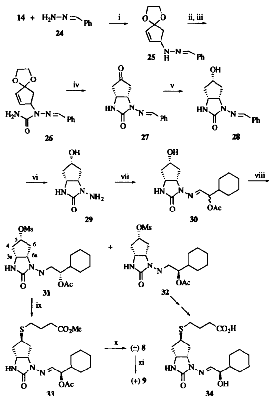
Scheme 2. Reagents: (i) Toluene -40^{\circ}\text{C} \rightarrow 0^{\circ}\text{C} ; \text{NEt}_3 , reflux 2 h (55%); (ii) \text{COCl}_2 , \text{C}_6\text{H}_5\text{N} , toluene 0^{\circ}\text{C} ; (iii) aqueous \text{NH}_3 (d 0.88) (90% overall); (iv) Camphor sulphonic acid, \text{Me}_2\text{CO} (55%); (v) \text{NaBH}_4 , EtOH (85%); (vi) \text{H}_2 , 10% Pd-C, EtOH, AcOH, 70^{\circ}\text{C} , 90 atmos (90%); (vii) \text{C}_6\text{H}_{11}\text{CH}(\text{OAc})\text{CHO} [ref. 30], NaOAc, MeOH, 50^{\circ}\text{C} , 3 h (75%); (viii) \text{MeSO}_2\text{Cl} , \text{C}_6\text{H}_5\text{N} , \text{CH}_2\text{Cl}_2 (35% of 31 , 36% of 32 ); (ix) Thiobutyrolactone, NaOMe, MeOH; DMSO (50%); (x) LiOH, \text{H}_2\text{O} -MeOH (86%); (xi) \text{Na}(\text{CN})\text{BH}_3 , AcOH, MeOH (90%).
